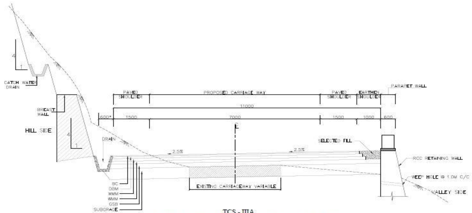
TCS - IIIA RECONSTRUCTION OF EXISTING CARRIAGEWAY WITH INTERMEDIATE SECTION IN RURAL SECTION
