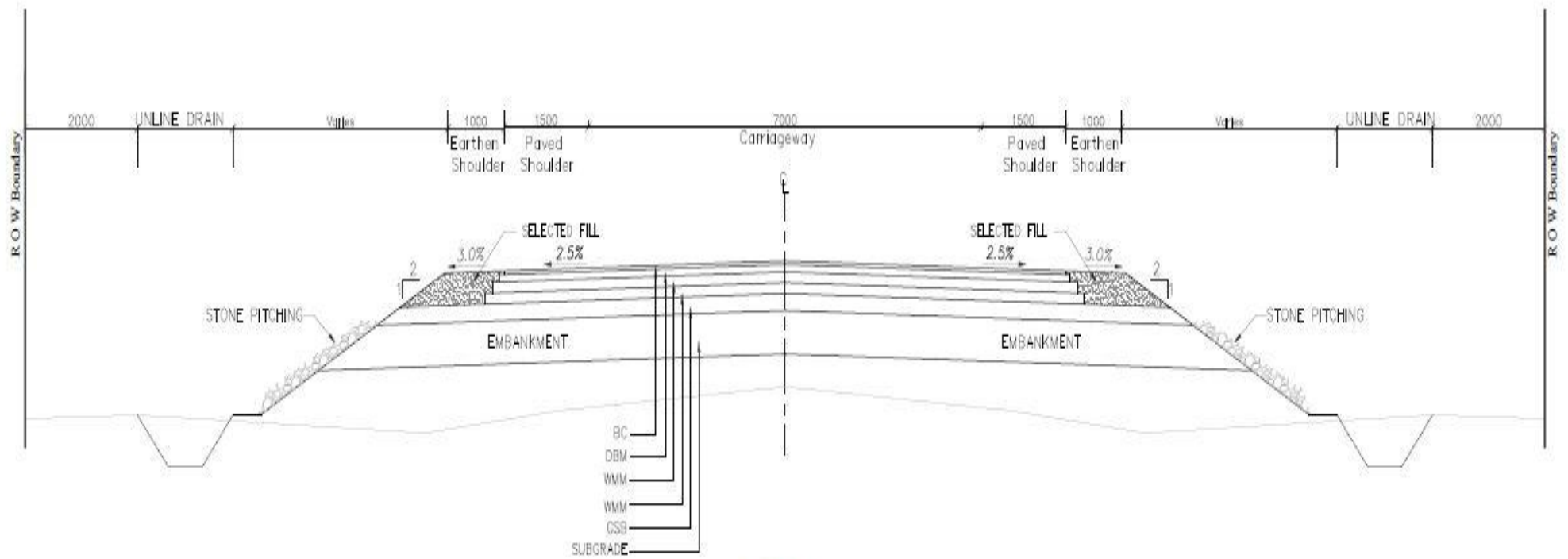
TCS - III D TWO LANE RAISING AT RIVERINE AREAS
